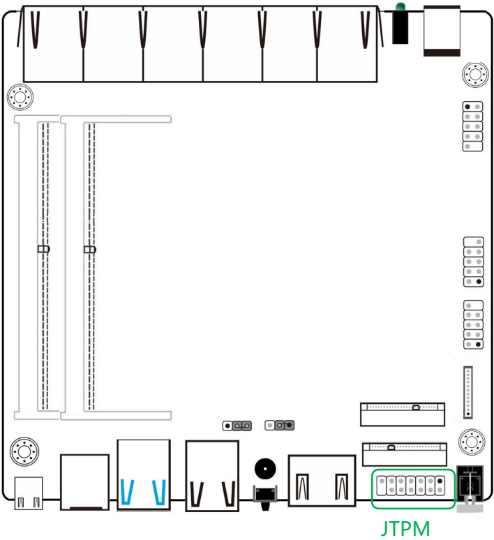
JTPM (2×7 pin 间距 2.00mm)
